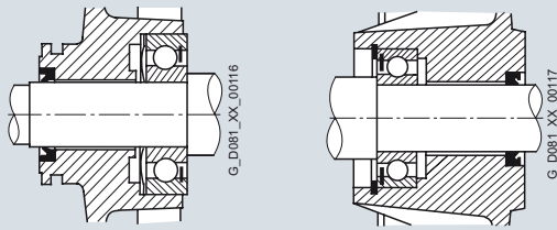
Fig. 10 Drive-end bearing Non-drive end bearing
