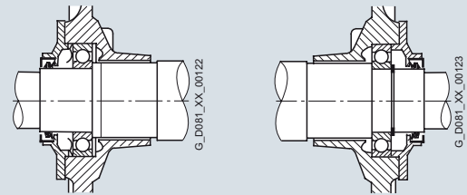
Fig. 11 Drive-end bearing Non-drive end bearing
