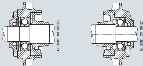
Fig. 12 Drive-end bearing Non-drive end bearing
