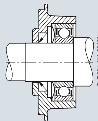
Fig. 2: Drive-end bearing
