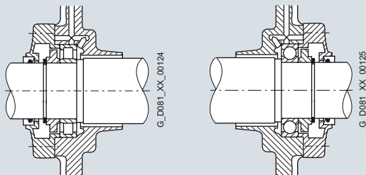
Fig. 12 Drive-end bearing Non-drive end bearing
